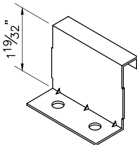
1 1/2" Fixed Mechanical Lock
